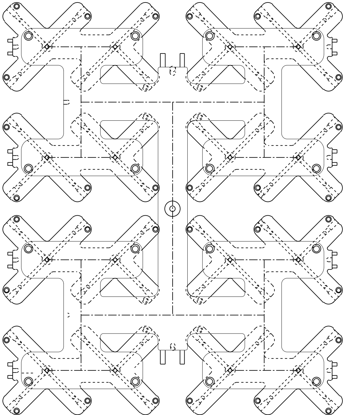
48-DROP BRIDGE MANIFOLD
